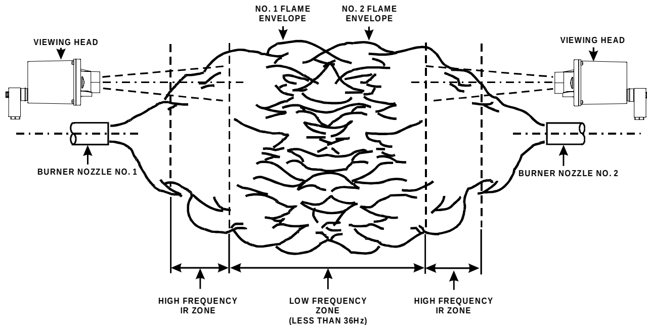
FIGURE 19 - OPPOSED FIRED VIEWING HEAD SIGHTING
