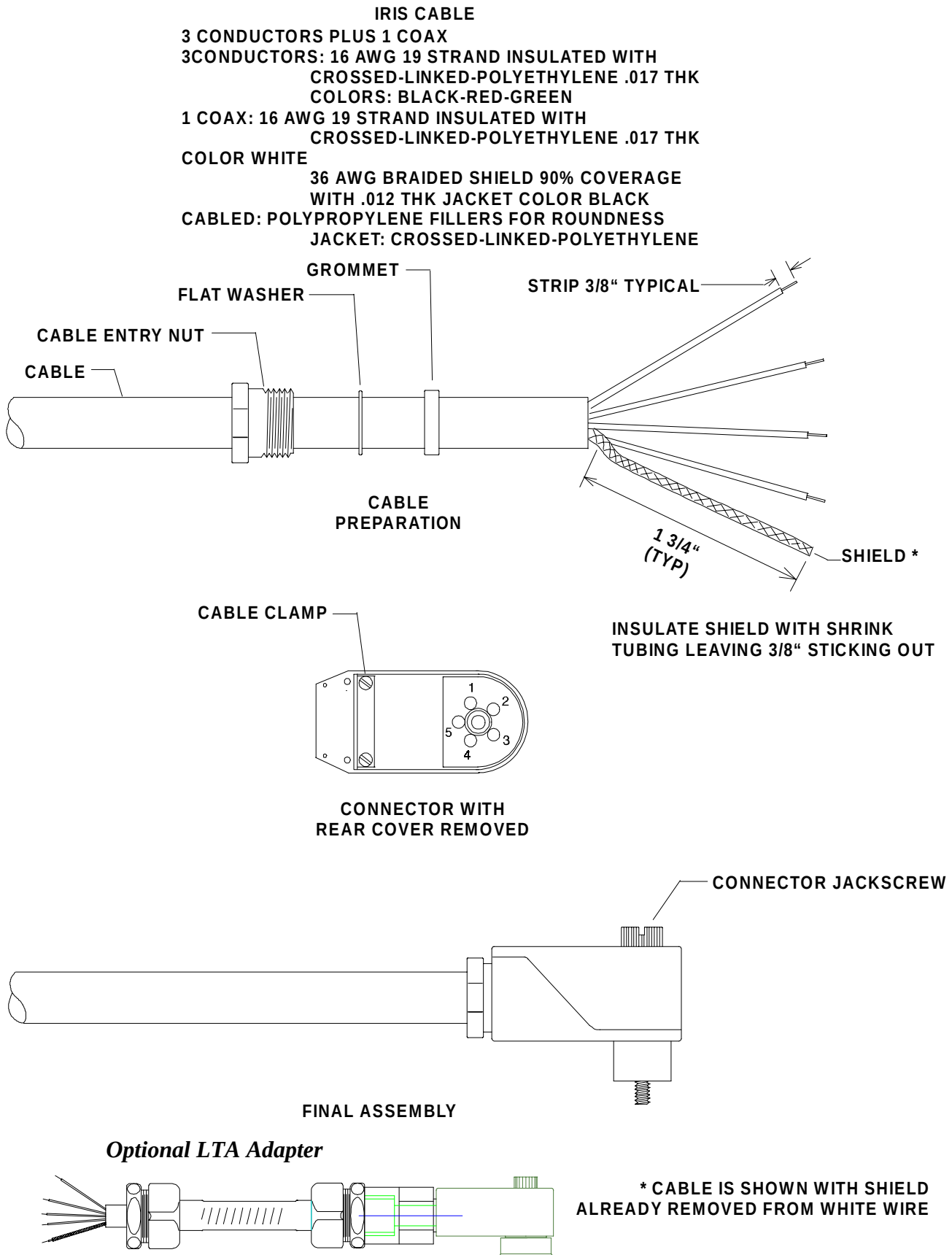
FIGURE 3 - WIRING AND ASSEMBLY - VIEWING HEAD
